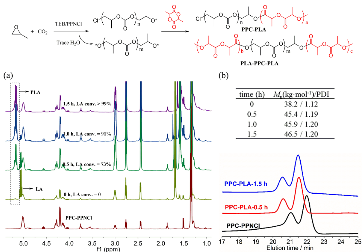
Figure 3. Synthesis of PPC-PLA block copolymers catalyzed by TEB/PPNCl: (a) evolution of 1 H NMR spectra of LA ROP with reaction time; (b) evolution of GPC traces and MWs.
