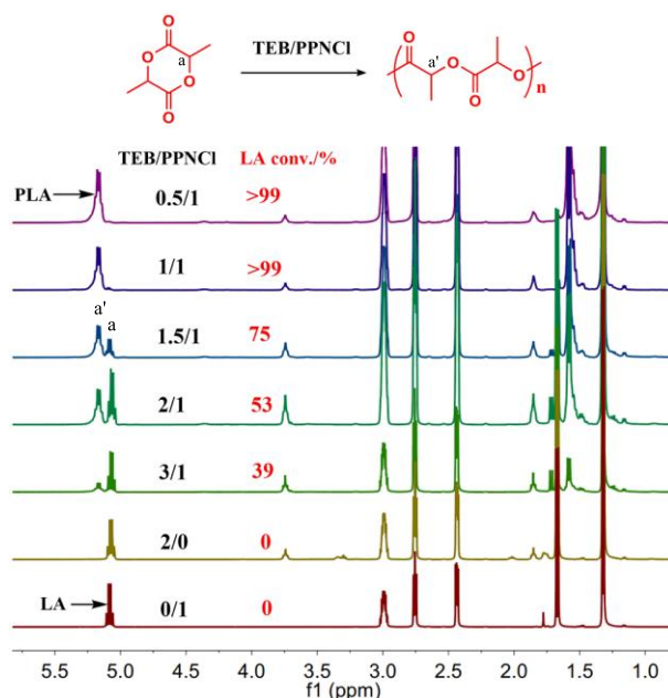
Figure 1. Evolution of ^1\text{H} NMR spectra for the copolymerization of PO/LA/PPNCl (500/100/1) catalyzed by different ratios of the TEB/PPNCl pair at 60 °C for 10 min.
